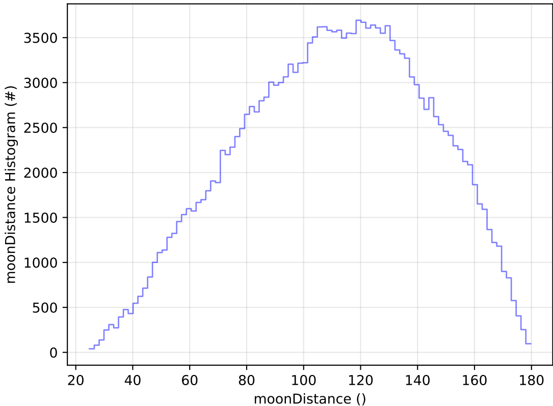
start_date_do90v3.4_10yrs All sky g band: moonDistance Histogram
