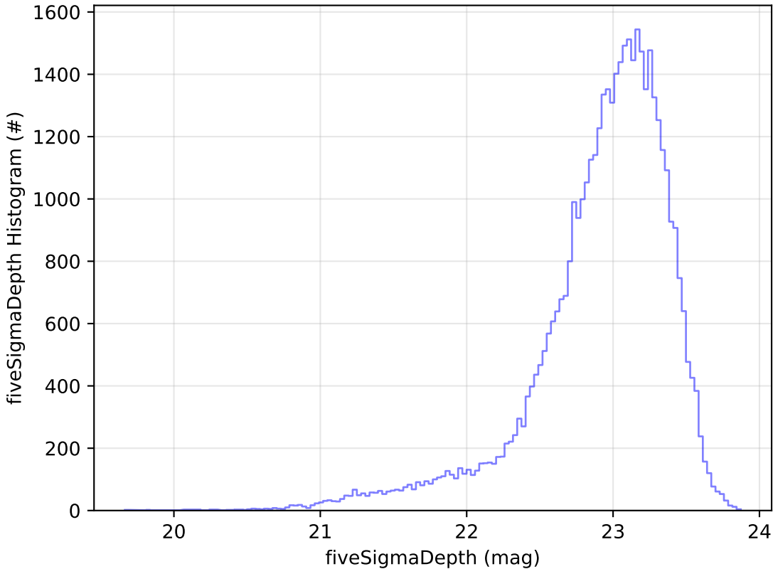
start_date_do90v3.4_10yrs Yr 1 z band: fiveSigmaDepth Histogram
