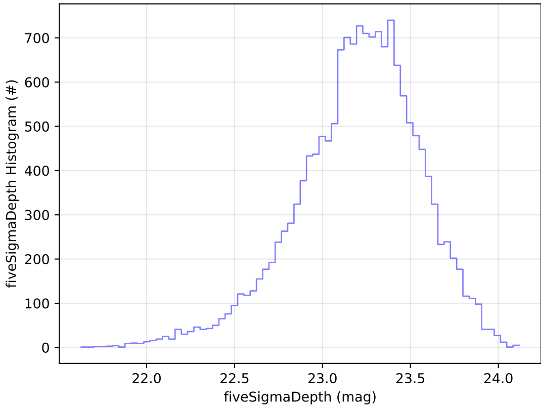
start_date_do90v3.4_10yrs Yr 1 u band: fiveSigmaDepth Histogram
