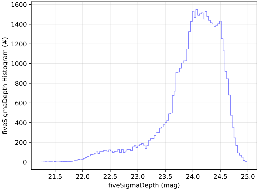
start_date_do90v3.4_10yrs Yr 1 r band: fiveSigmaDepth Histogram
