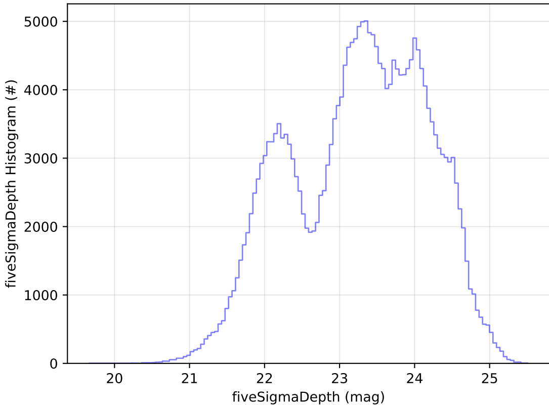
start_date_do90v3.4_10yrs Yr 1 all bands: fiveSigmaDepth Histogram
