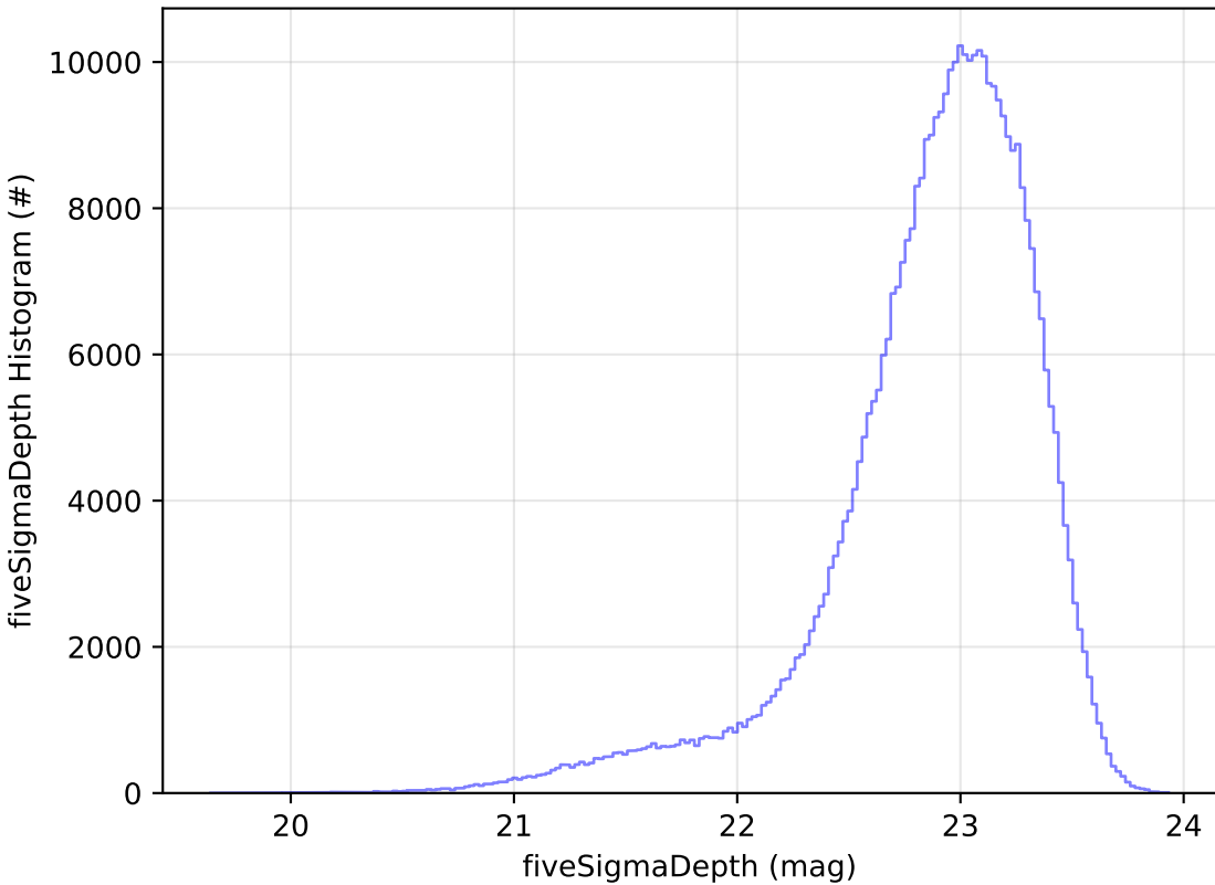
start_date_do90v3.4_10yrs WFD z band: fiveSigmaDepth Histogram
