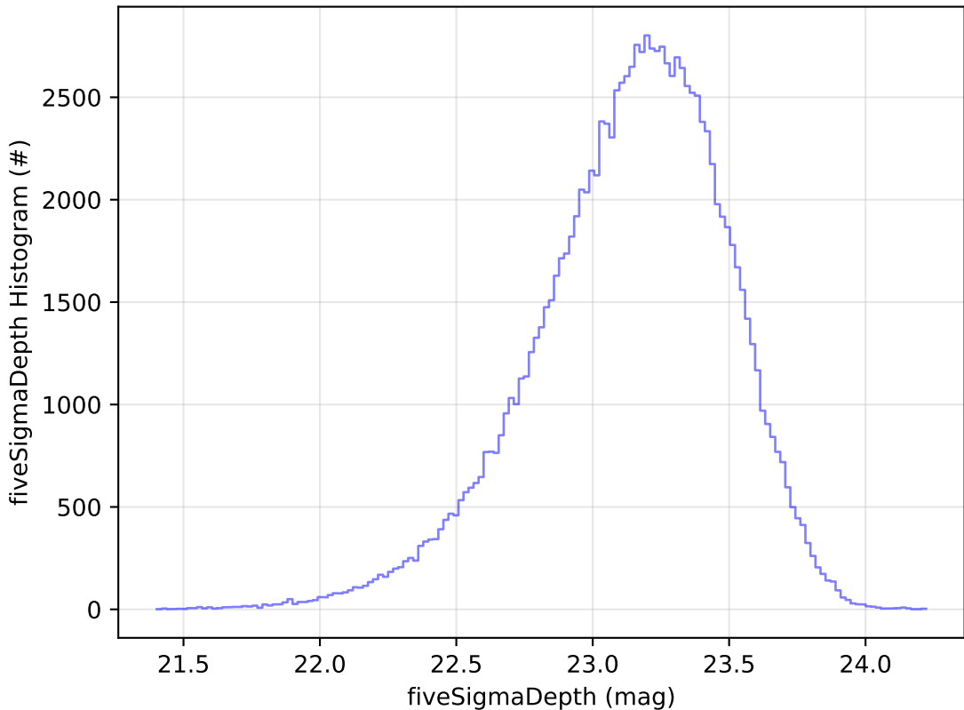
start_date_do90v3.4_10yrs WFD u band: fiveSigmaDepth Histogram
