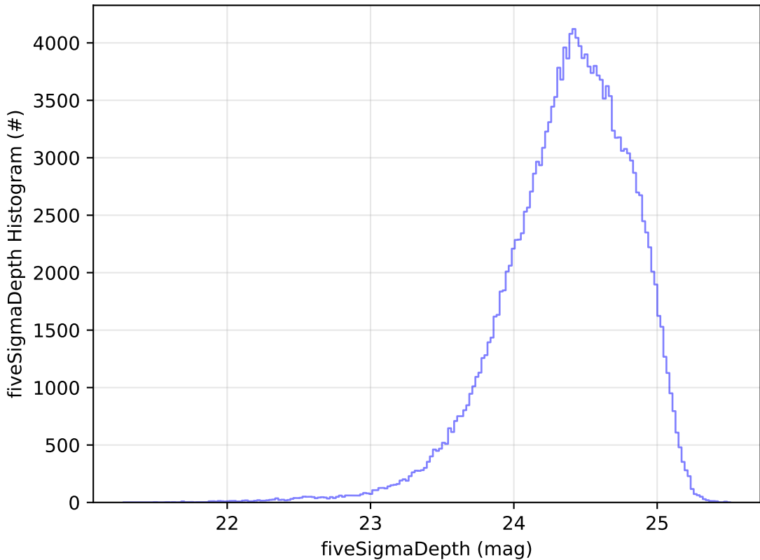
start_date_do90v3.4_10yrs WFD g band: fiveSigmaDepth Histogram
