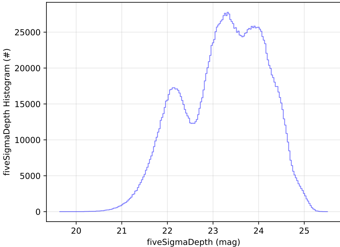
start_date_do90v3.4_10yrs WFD all bands: fiveSigmaDepth Histogram
