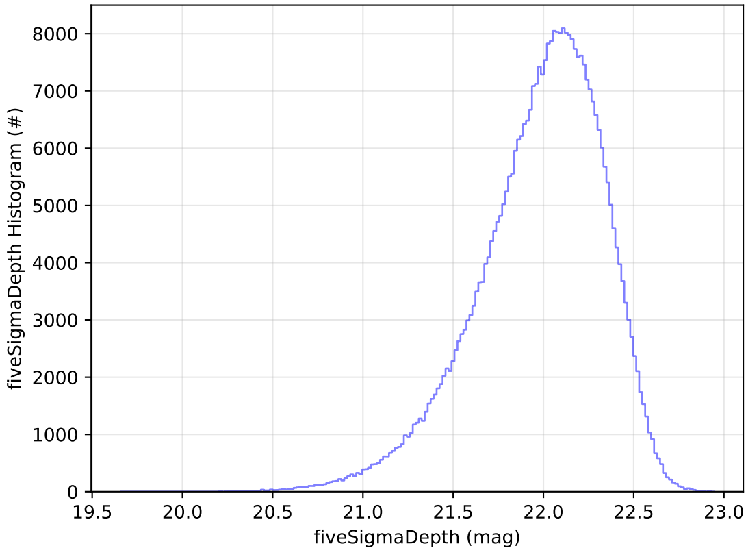
start_date_do90v3.4_10yrs All sky y band: fiveSigmaDepth Histogram
