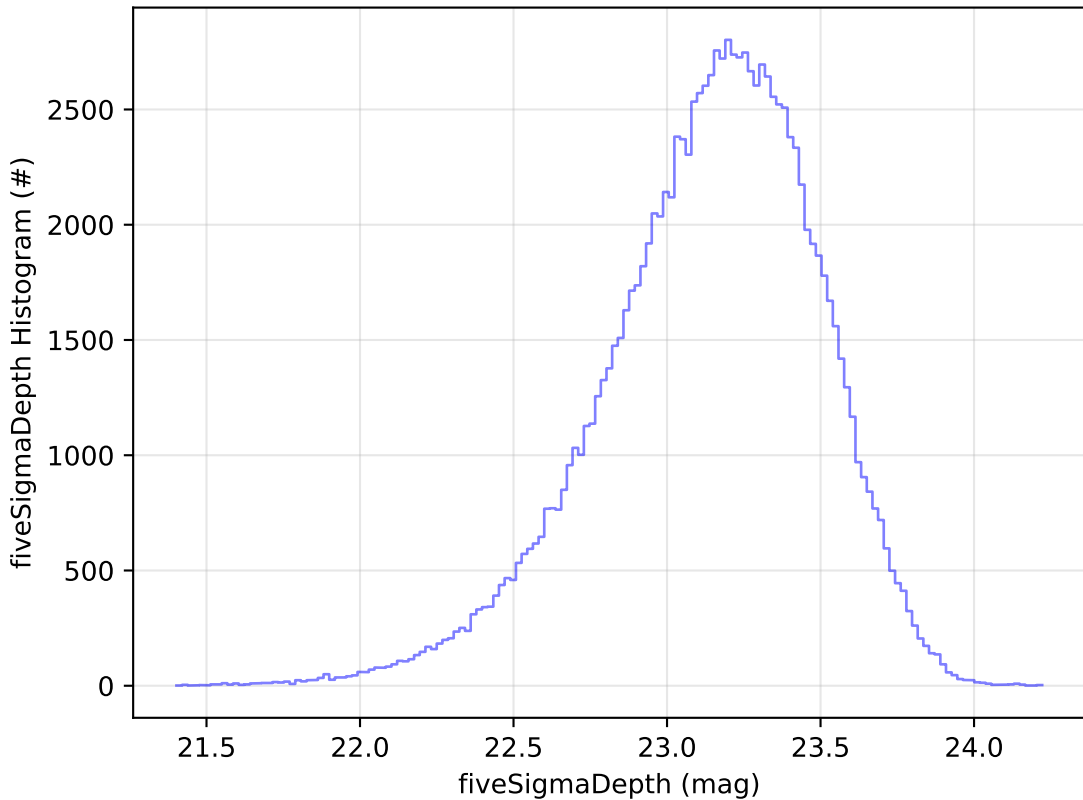
start_date_do90v3.4_10yrs All sky u band: fiveSigmaDepth Histogram
