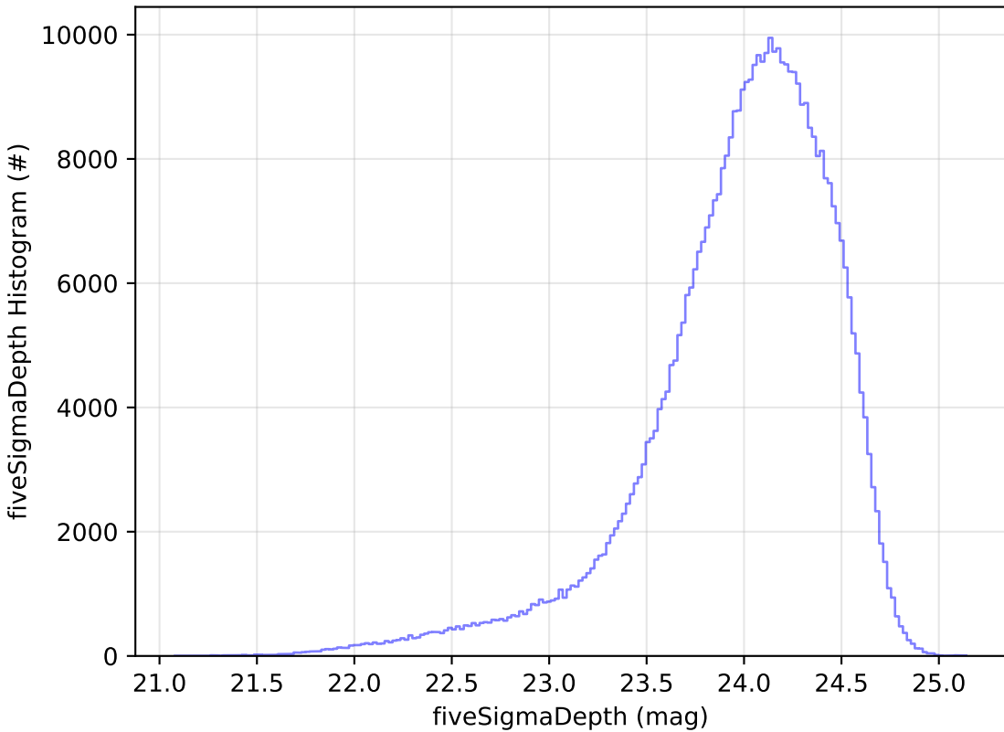
start_date_do90v3.4_10yrs All sky r band: fiveSigmaDepth Histogram
