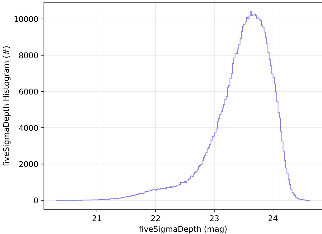
start_date_do90v3.4_10yrs All sky i band: fiveSigmaDepth Histogram
