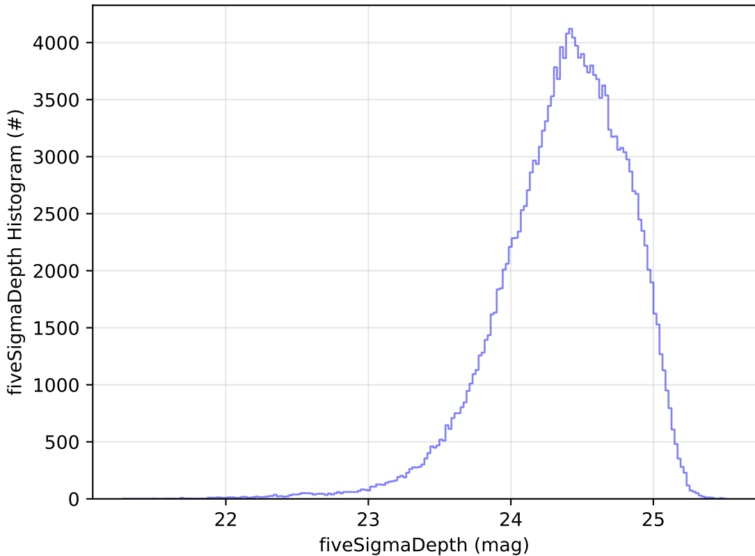
start_date_do90v3.4_10yrs All sky g band: fiveSigmaDepth Histogram
