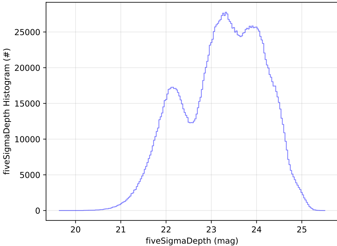
start_date_do90v3.4_10yrs All sky all bands: fiveSigmaDepth Histogram
