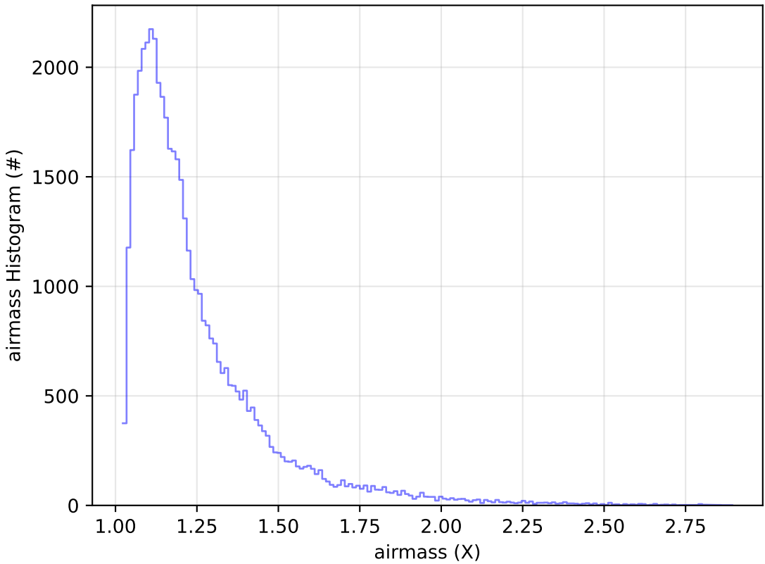
start_date_do90v3.4_10yrs Yr 1 y band: airmass Histogram
