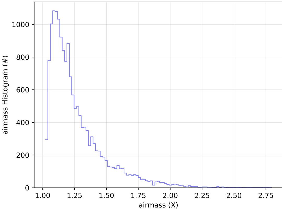
start_date_do90v3.4_10yrs Yr 1 u band: airmass Histogram
