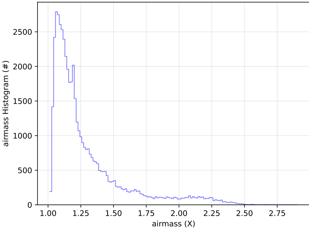
start_date_do90v3.4_10yrs Yr 1 r band: airmass Histogram
