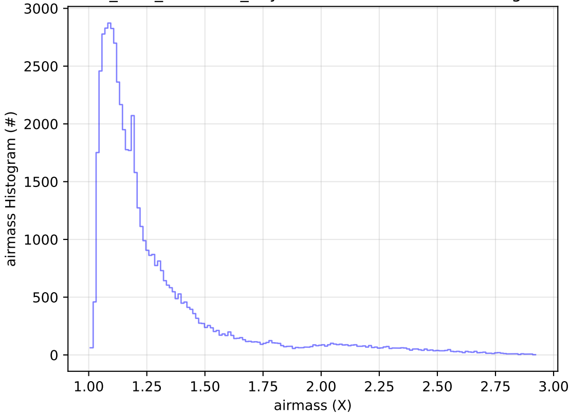
start_date_do90v3.4_10yrs Yr 1 i band: airmass Histogram
