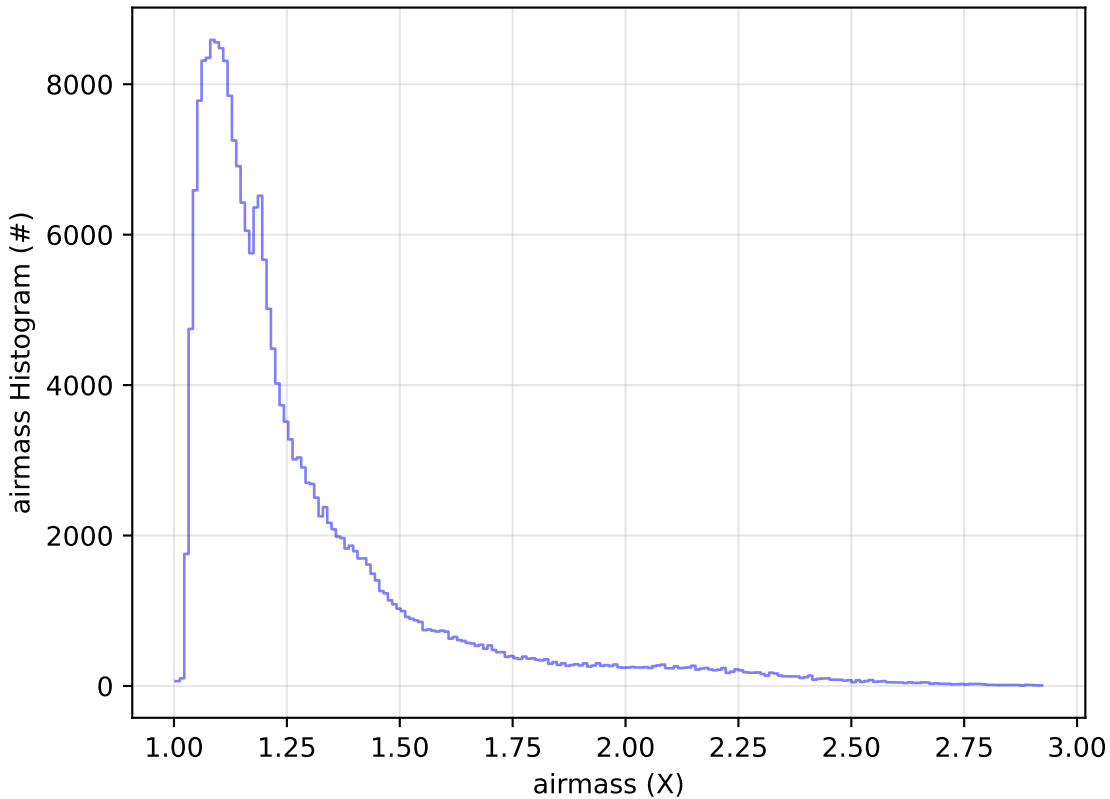
start_date_do90v3.4_10yrs Yr 1 all bands: airmass Histogram
