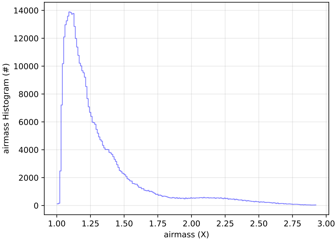
start_date_do90v3.4_10yrs WFD z band: airmass Histogram
