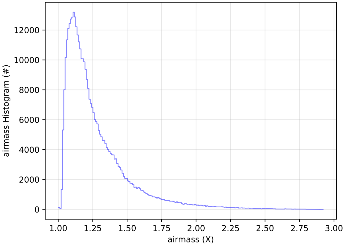
start_date_do90v3.4_10yrs WFD y band: airmass Histogram
