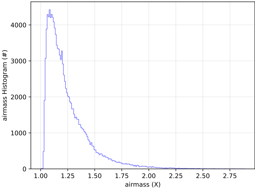
start_date_do90v3.4_10yrs WFD u band: airmass Histogram
