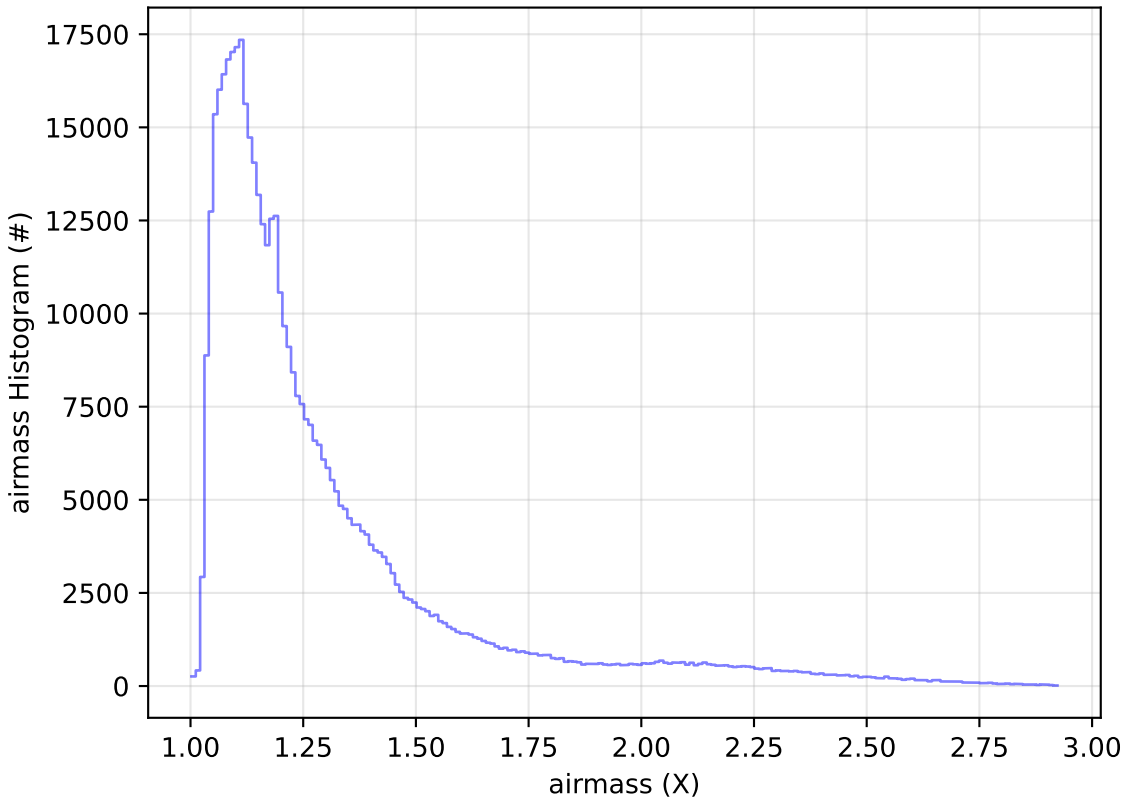
start_date_do90v3.4_10yrs WFD i band: airmass Histogram
