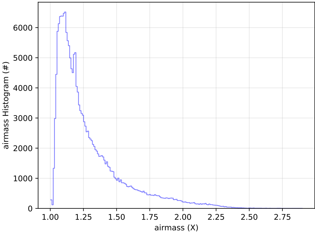
start_date_do90v3.4_10yrs WFD g band: airmass Histogram
