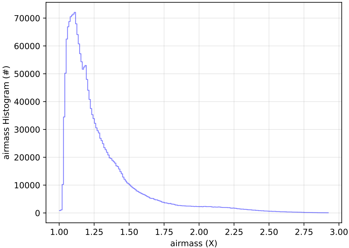
start_date_do90v3.4_10yrs WFD all bands: airmass Histogram
