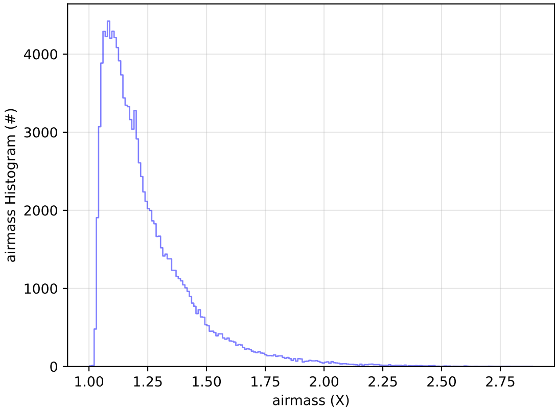
start_date_do90v3.4_10yrs All sky u band: airmass Histogram
