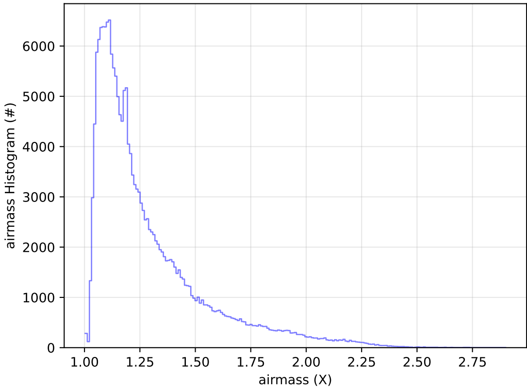
start_date_do90v3.4_10yrs All sky g band: airmass Histogram
