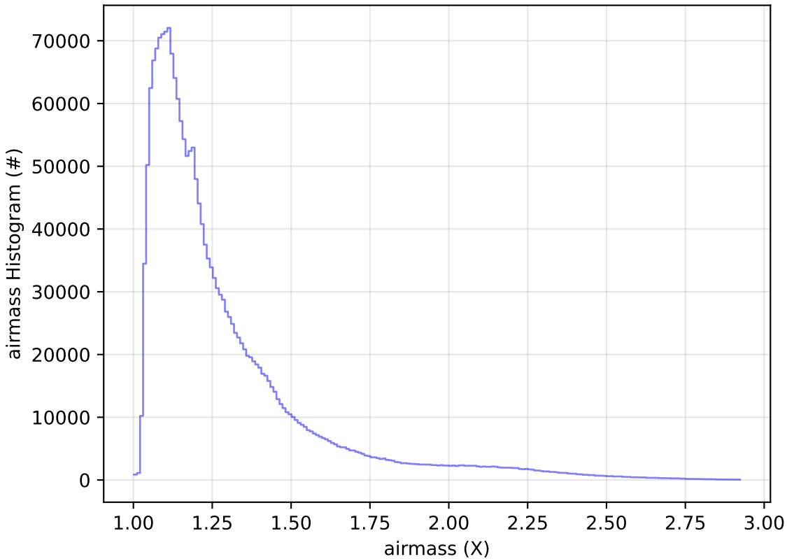
start_date_do90v3.4_10yrs All sky all bands: airmass Histogram
