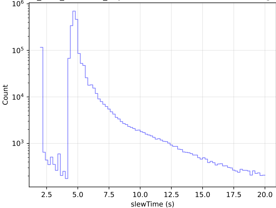
start_date_do90v3.4_10yrs All visits: Zoom Slew Time Histogram
