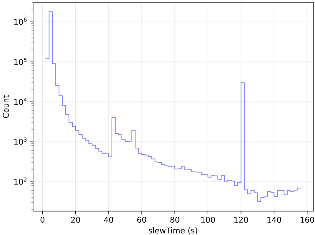
start_date_do90v3.4_10yrs All visits: Slew Time Histogram
