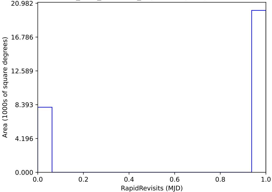
start_date_do90v3.4_10yrs All sky: RapidRevisits
