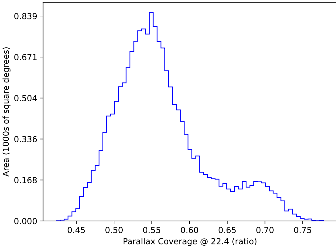
start_date_do90v3.4_10yrs WFD: Parallax Coverage @ 22.4
