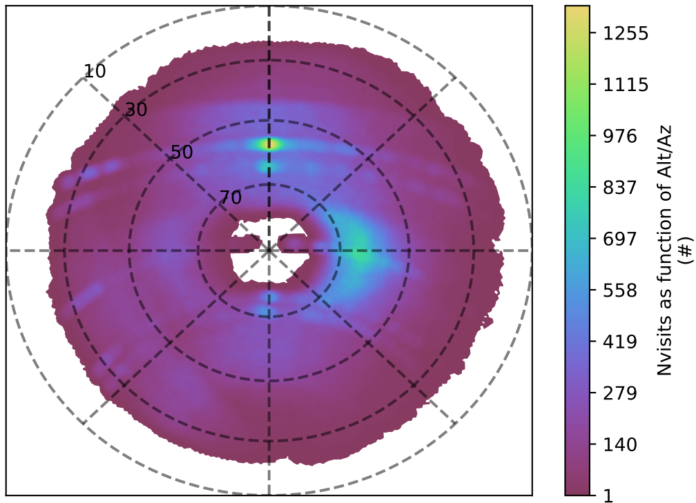
start_date_do90v3.4_10yrs g band: Nvisits as function of Alt/Az
