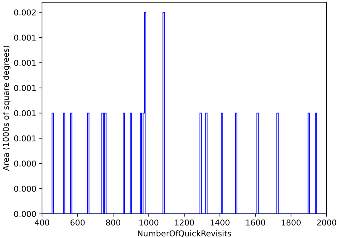
start_date_do90v3.4_10yrs WFD: NumberOfQuickRevisits
