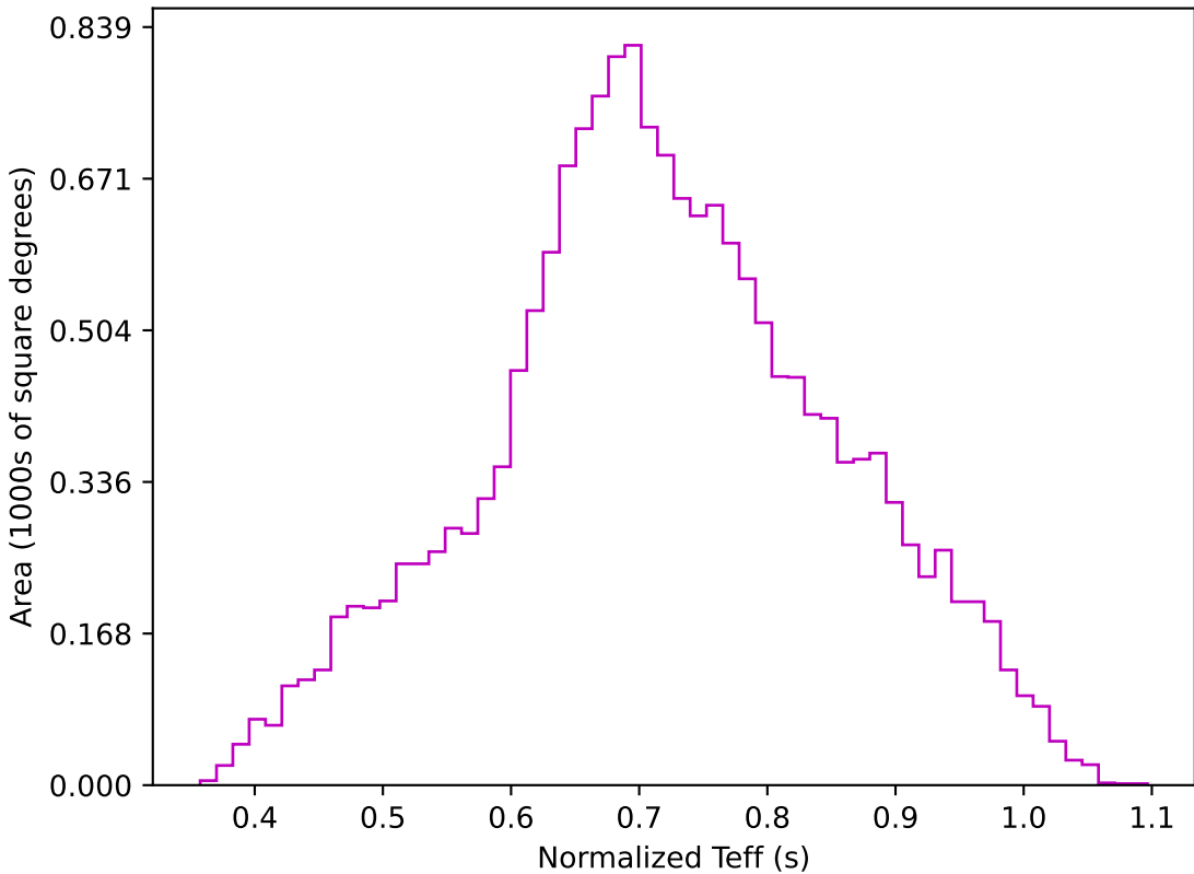
start_date_do90v3.4_10yrs WFD z band: Normalized Teff
