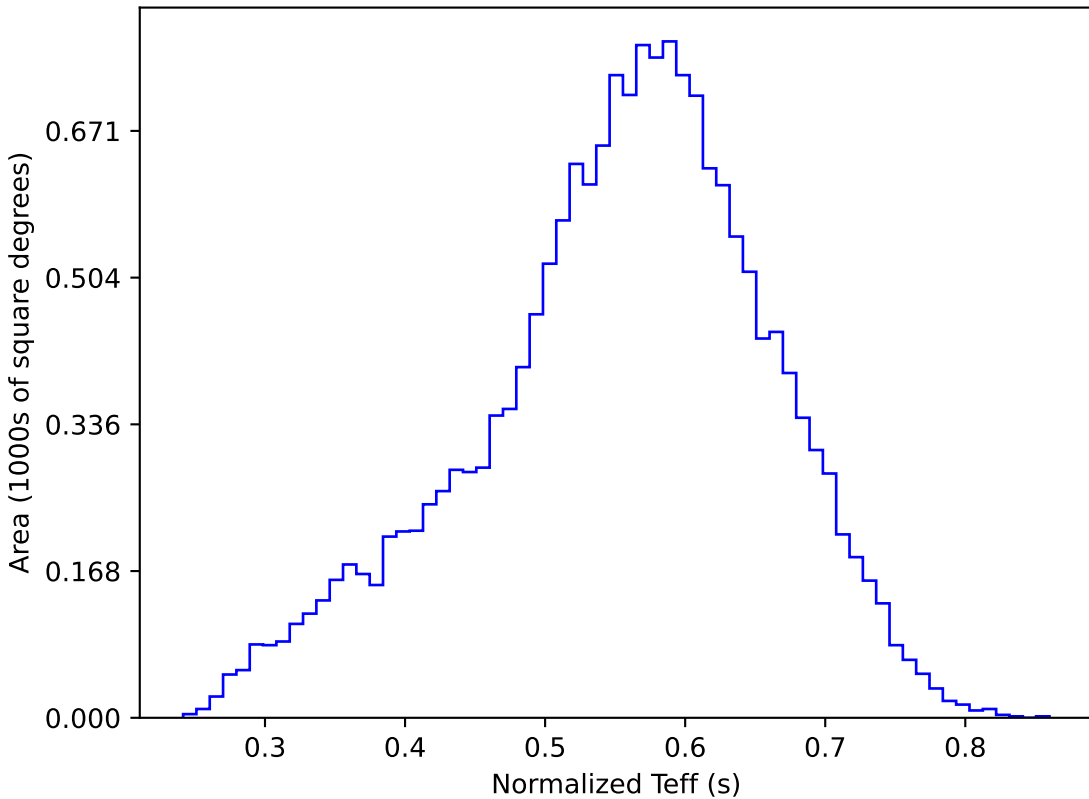
start_date_do90v3.4_10yrs WFD y band: Normalized Teff
