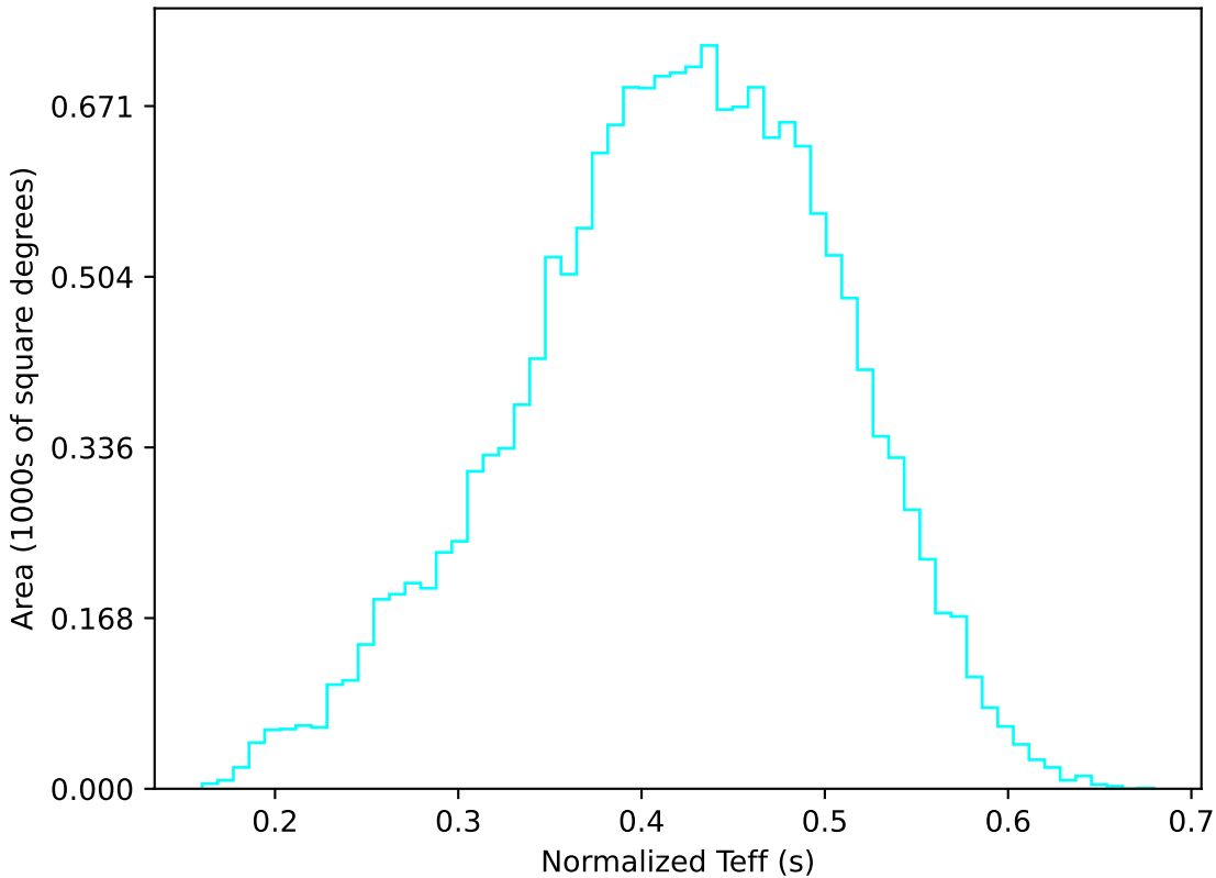
start_date_do90v3.4_10yrs WFD u band: Normalized Teff
