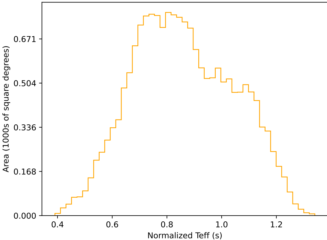
start_date_do90v3.4_10yrs WFD r band: Normalized Teff
