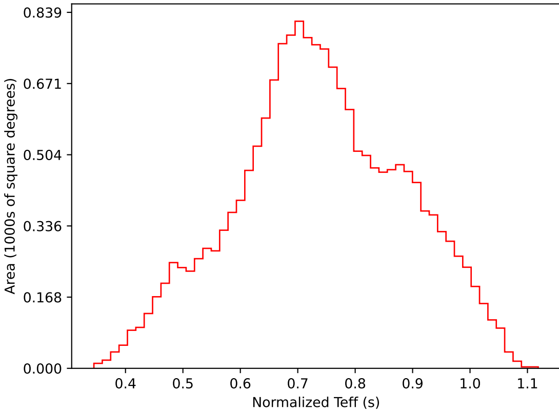
start_date_do90v3.4_10yrs WFD i band: Normalized Teff
