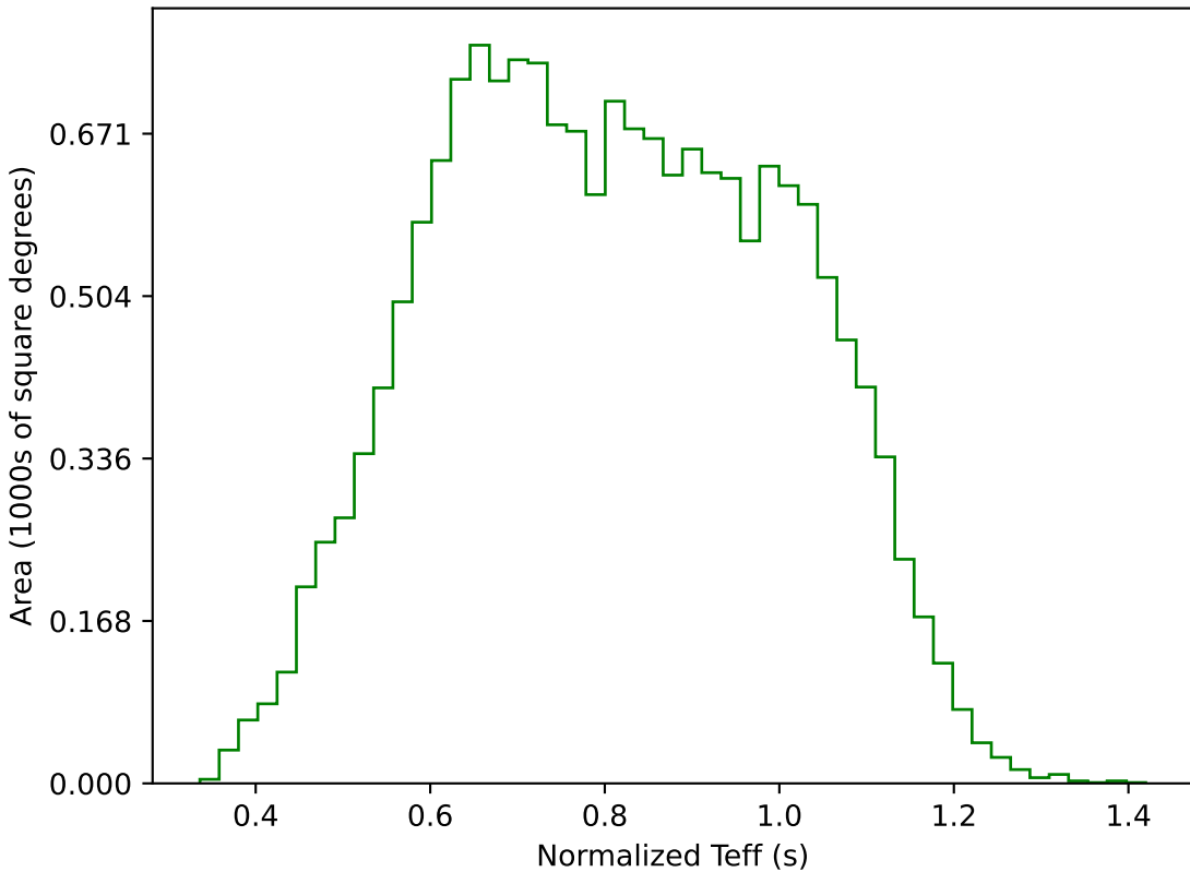
start_date_do90v3.4_10yrs WFD g band: Normalized Teff
