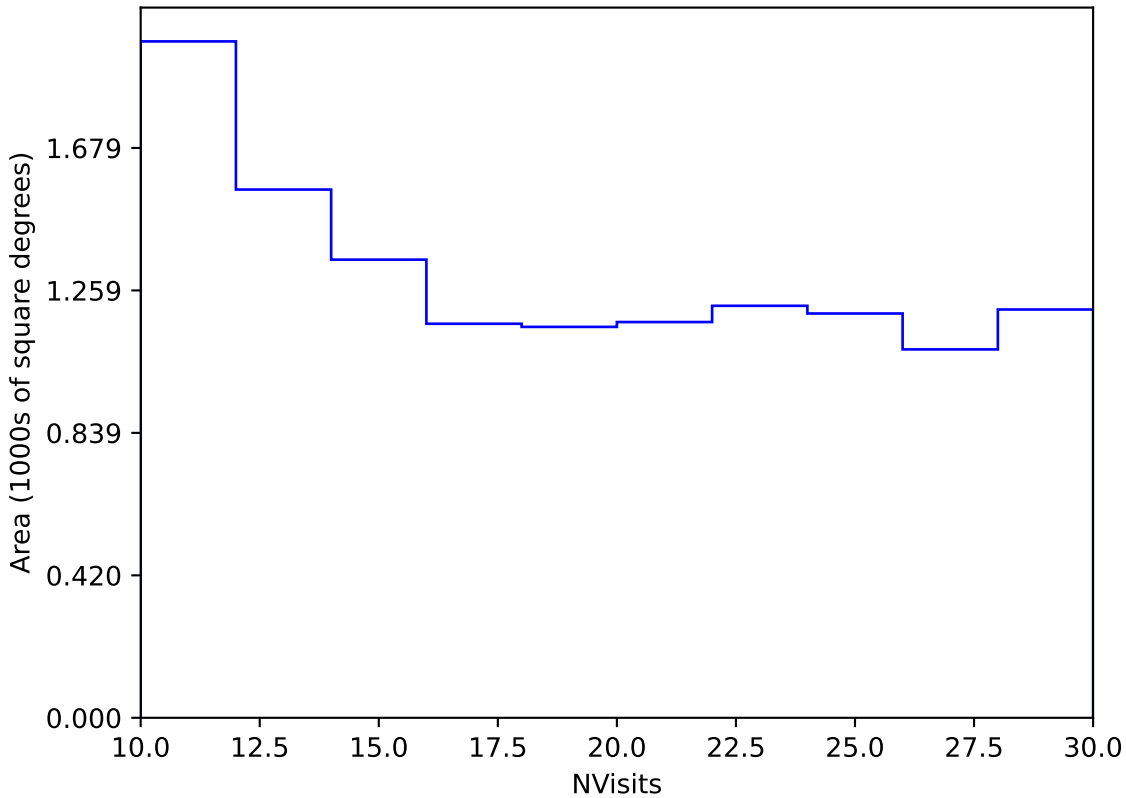
start_date_do90v3.4_10yrs Yr 3-4 y band: NVisits
