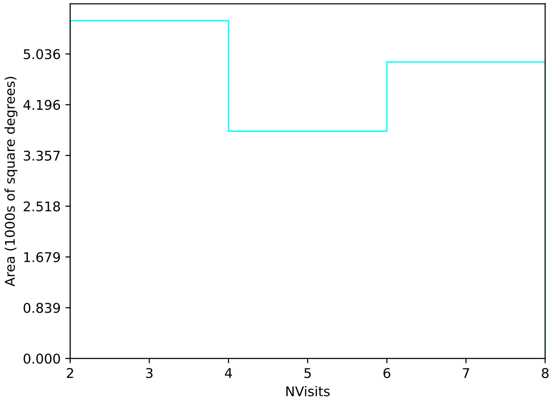
start_date_do90v3.4_10yrs Yr 3-4 u band: NVisits
