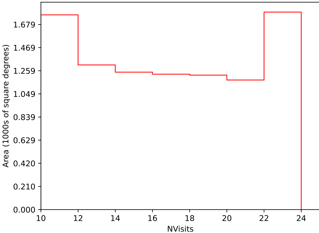
start_date_do90v3.4_10yrs Yr 3-4 i band: NVisits
