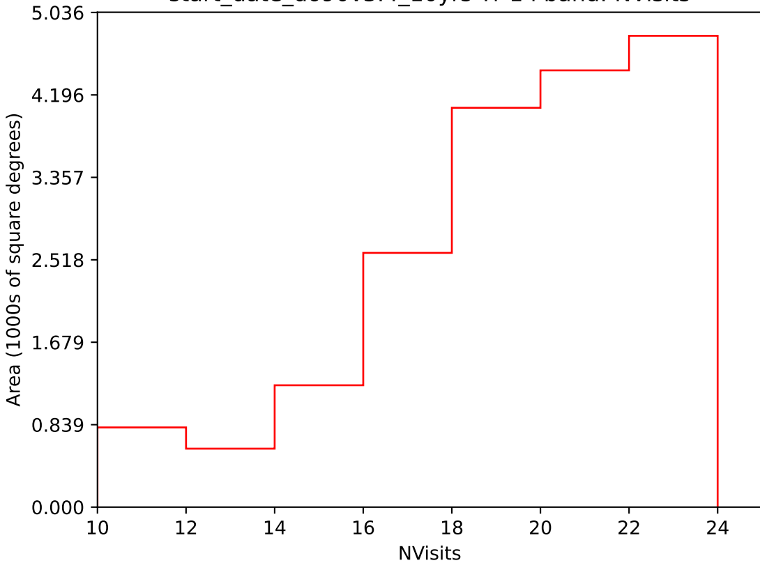
start_date_do90v3.4_10yrs Yr 1 i band: NVisits
