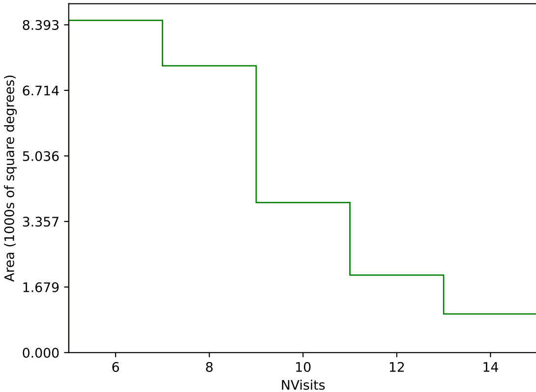
start_date_do90v3.4_10yrs Yr 1 g band: NVisits
