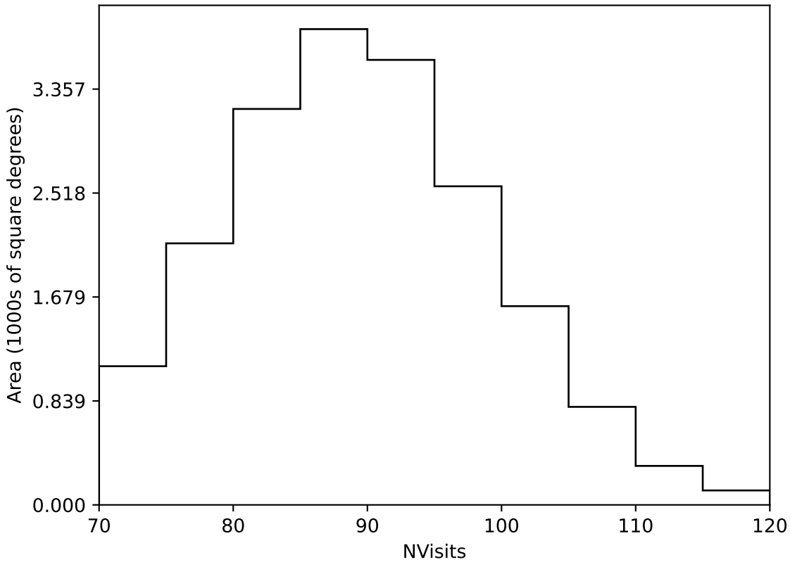
start_date_do90v3.4_10yrs Yr 1 all bands: NVisits
