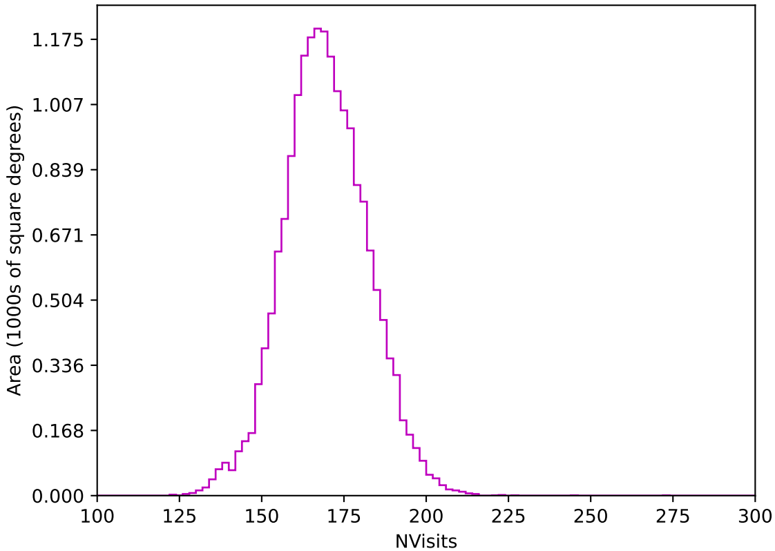
start_date_do90v3.4_10yrs WFD z band: NVisits
