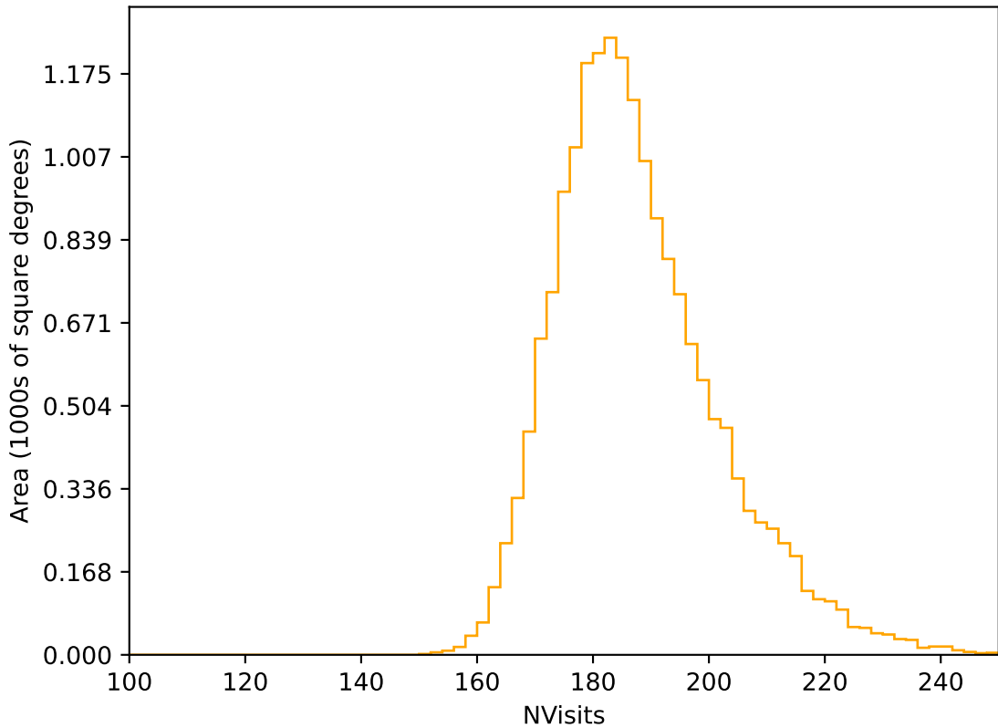
start_date_do90v3.4_10yrs WFD r band: NVisits
