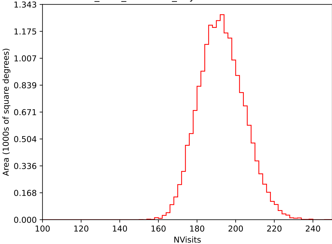
start_date_do90v3.4_10yrs WFD i band: NVisits
